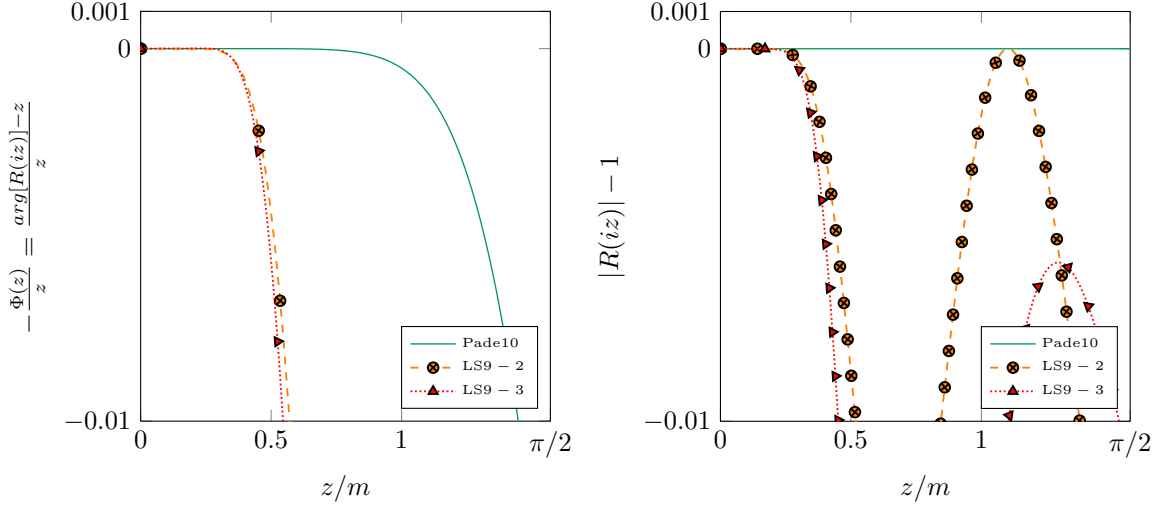
Figure 5: Dispersion and dissipation curves of diagonal Padé schemes of order 10 compared with that of the Linear-SDIRK, when applied to the test equation (11). LS9 – l represents the s = 9 plus l additional stages Linear-SDIRK of order 10.
