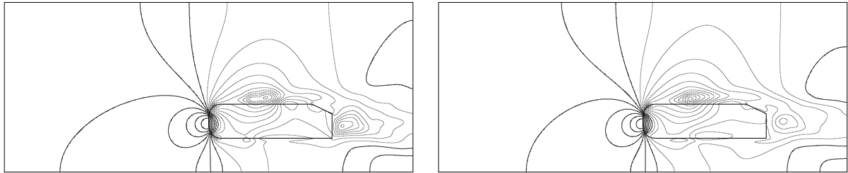
Figure 12: Mean pressure isolines for the flow around Ahmed body with a rear window on top of a road at Re_L = 30000 . Cases 0 (left) and 4 (right).
