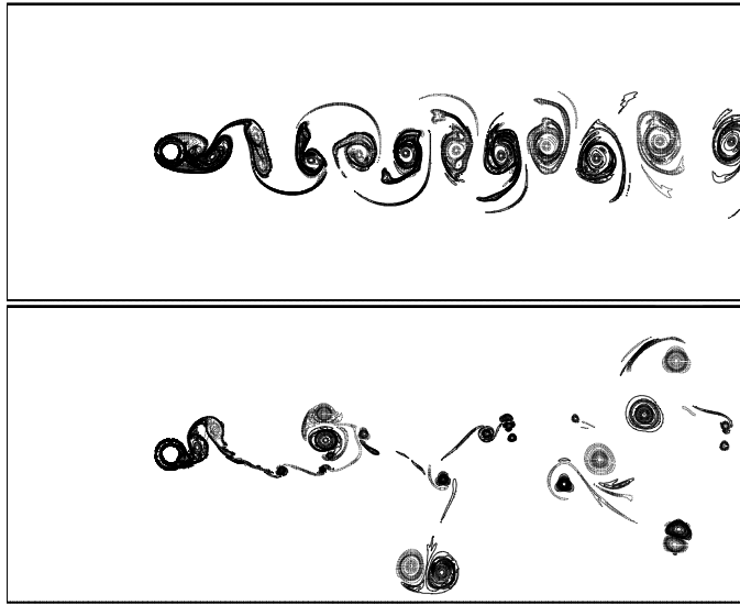
Figure 6: Vorticity field with (top) and without (bottom) control for the same time at Re_D = 24000 .
