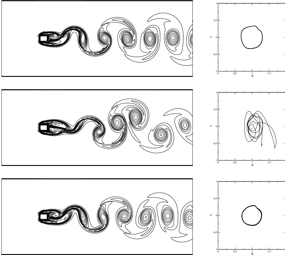
Figure 3: Comparison of vorticity fields and phase portraits at monitoring point (4.0625, 0.75) for Re_H = 300 with (top) and without (middle) control in an open domain. The figures at the bottom concern an uncontrolled flow at Re_H = 250 .
