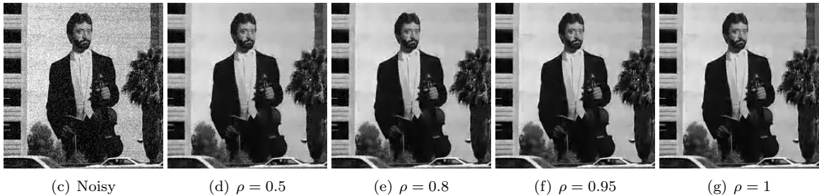
Supplemental Figure 2: Top: PSNR as a function of speed-up for varying values of the proportion \rho used in the flat tail approximation when (a) no other accelerations are used and (b) the other two accelerations are also used. The parameter offering the best speed-up for a drop of at most -0.2\text{dB} is indicated. Bottom: (c) a noisy image with \sigma=20 and (d-g) FEPLL results obtained for increasing value of \rho (includes the other two accelerations as well).
