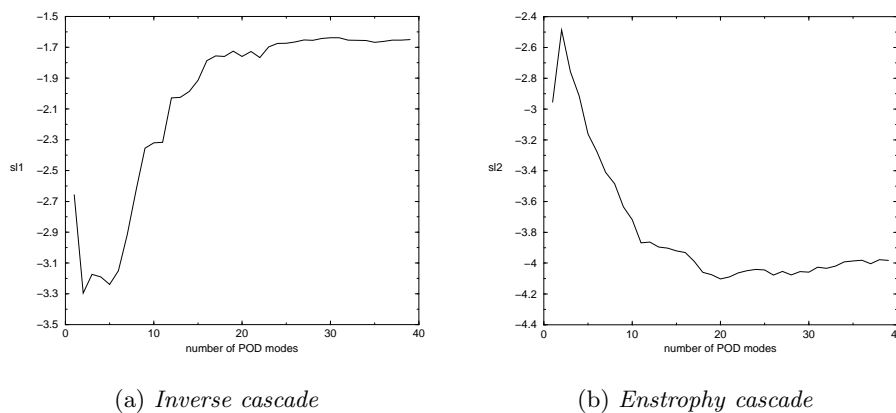
Figure 22: Evolution of the slopes in function of the number of POD modes in the reconstruction
