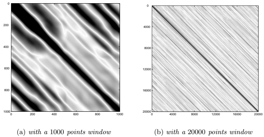
Figure 13: The correlation matrices for different time windows calculated for the first component of the velocity
