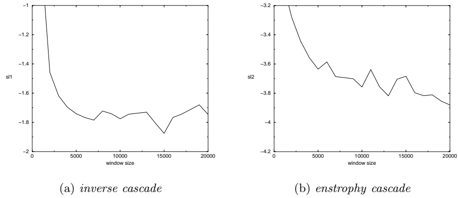
Figure 12: Slope estimates computed with the Welch correlation method in terms of the window size
