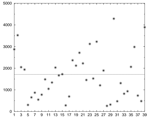
Figure 17: POD modes for the vorticity signal
