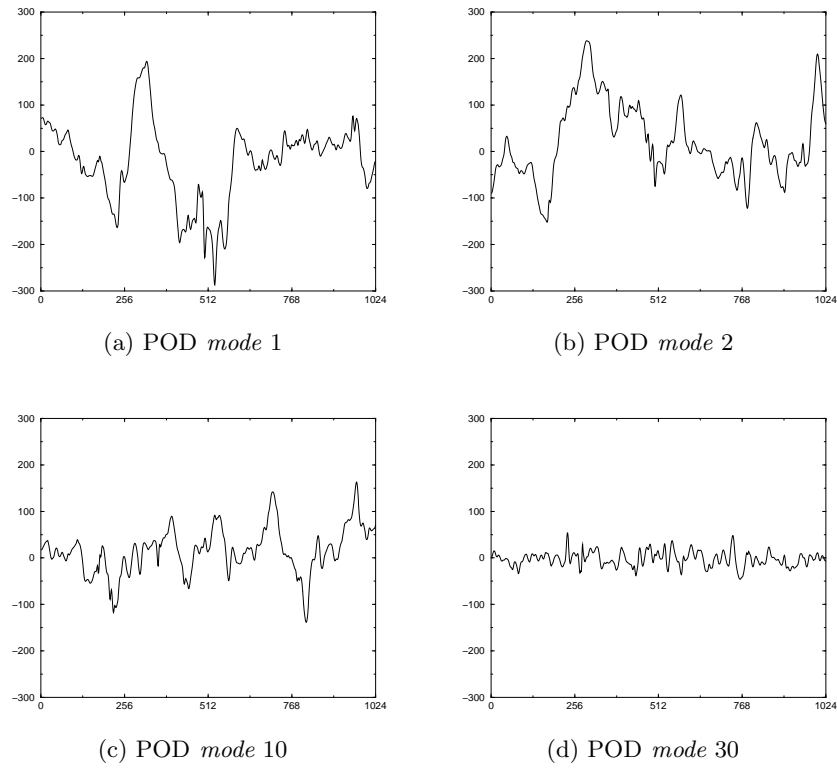
Figure 17: POD modes for the vorticity signal
