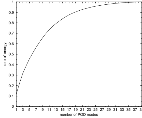
Figure 19: Quality of the reconstruction versus the number of POD modes
