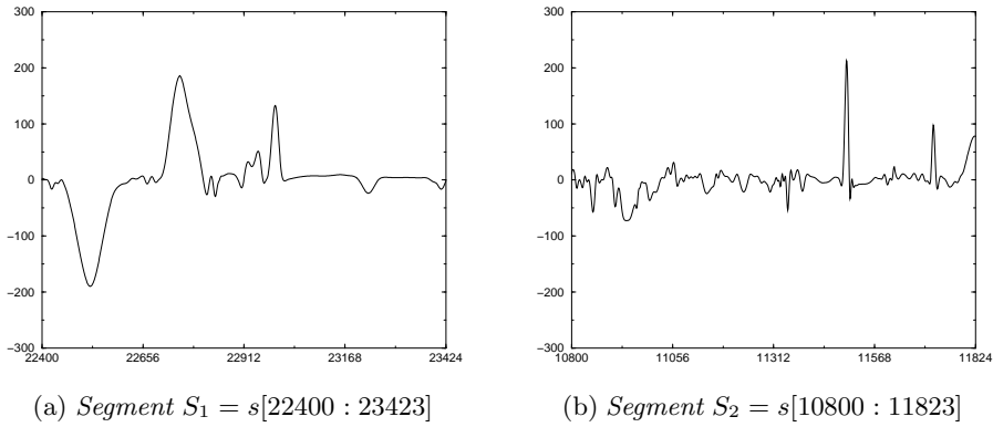
Figure 20: Randomly chosen segments of the vorticity signal
