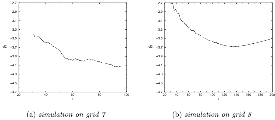
Figure 5: Determination of the upper bound to evaluate the enstrophy cascade slope
