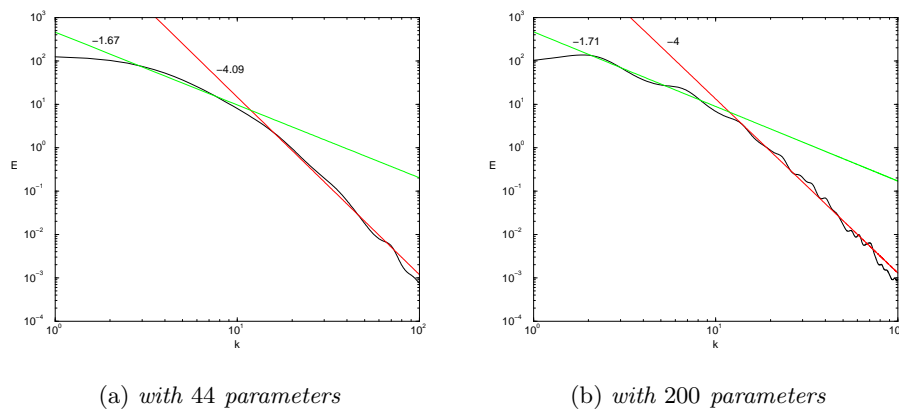
Figure 14: Energy spectra obtained by the autoregressive method with different parameters
