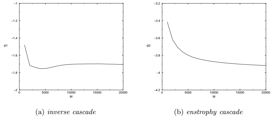
Figure 10: Slope estimates computed with the correlation method in terms of M
