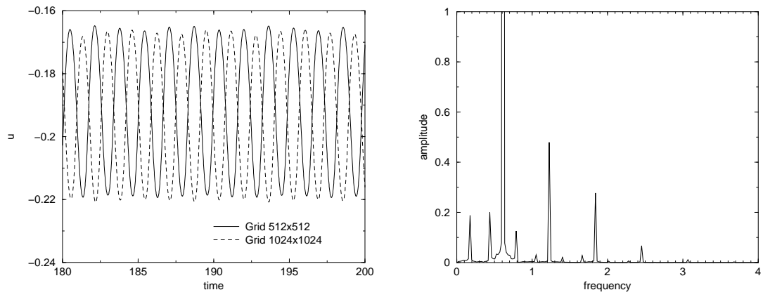
Fig. 7. Horizontal velocity history (left) and power spectrum (right) at monitoring point (14/16, 13/16) for Re = 10000 . Computation with Gear scheme in time and present scheme in space.
