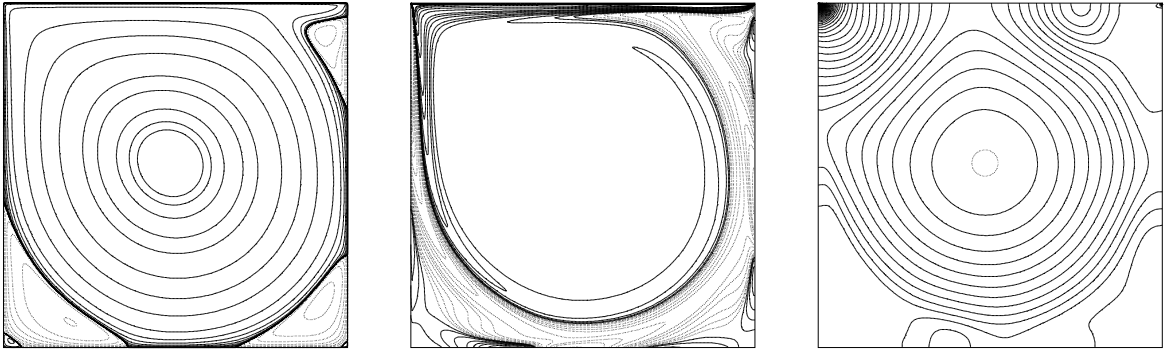
Fig. 3. Steady solution at Re = 5000 computed with present scheme on grid 2048 \times 2048 . From left to right stream-function, vorticity and pressure fields.
