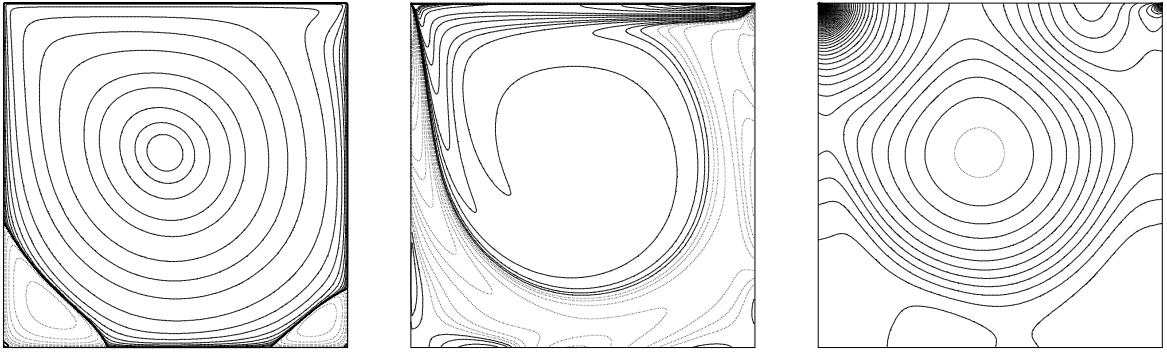
Fig. 2. Steady solution at Re = 1000 computed with present scheme on grid 1024 \times 1024 . From left to right stream-function, vorticity and pressure fields.
