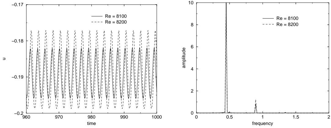
Fig. 6. Horizontal velocity history (left) and power spectrum (right) on grid 512 \times 512 at monitoring point (14/16, 13/16) for Re = 8100 and Re = 8200 . Computation with Gear scheme in time and present scheme in space.
