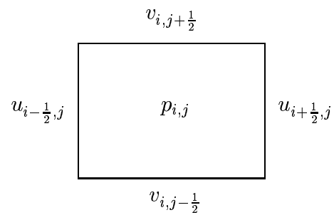
Fig. 1. A staggered cell
