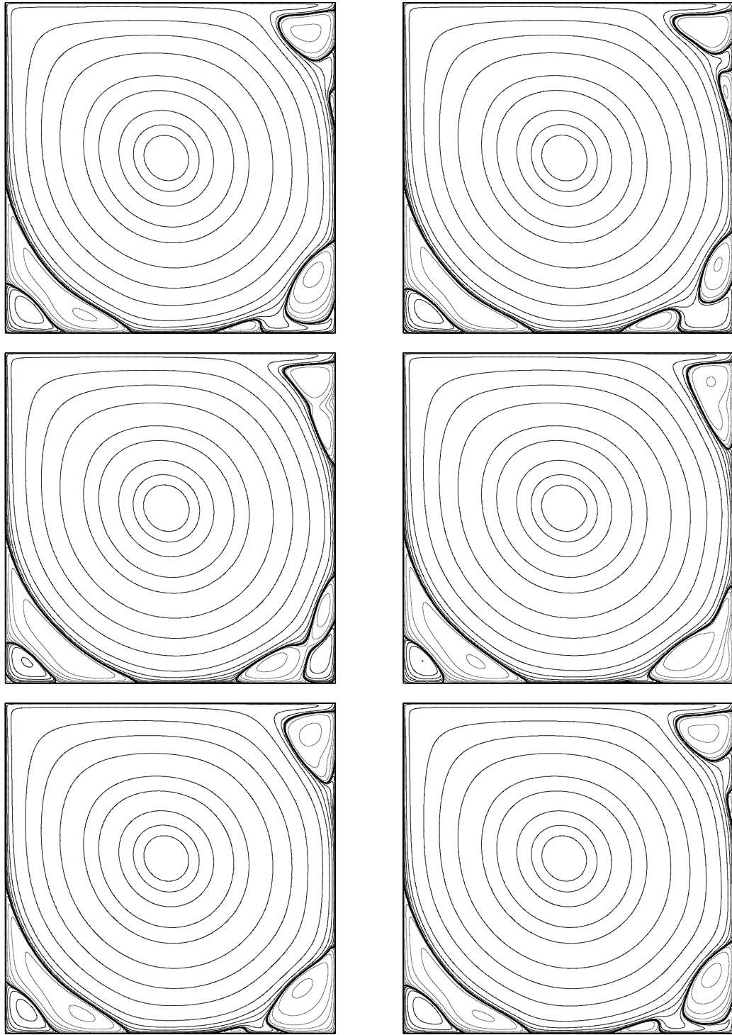
Fig. 9. Evolution of the streamfunction during one main period for Re = 10000 on grid 1024 \times 1024 . From top to bottom and left to right are represented times t = 0 , t = 0.328 , t = 0.656 , t = 0.984 , t = 1.312 and t = 1.64 .
