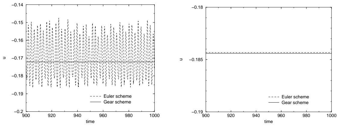
Fig. 4. Horizontal velocity history at monitoring point (14/16, 13/16) for Re = 7800 . Comparison of Euler and Gear schemes on the 128 \times 128 (left) and 256 \times 256 (right) grids.
