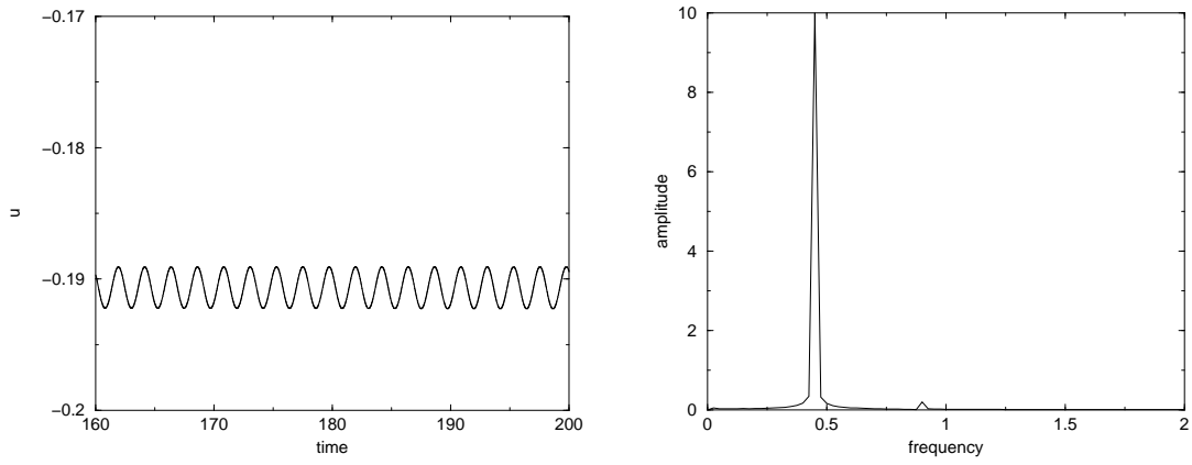
Fig. 5. Horizontal velocity history (left) and power spectrum (right) on grid 1024 \times 1024 at monitoring point (14/16, 13/16) for Re = 8050 . Computation with Gear scheme in time and present scheme in space.
