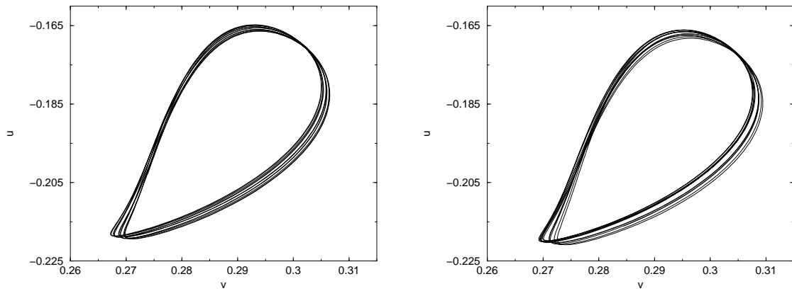
Fig. 8. Phase portrait on grid 512 \times 512 (left) and on grid 1024 \times 1024 (right) at monitoring point (14/16, 13/16) for Re = 10000 . Computation with Gear scheme in time and present scheme in space.
