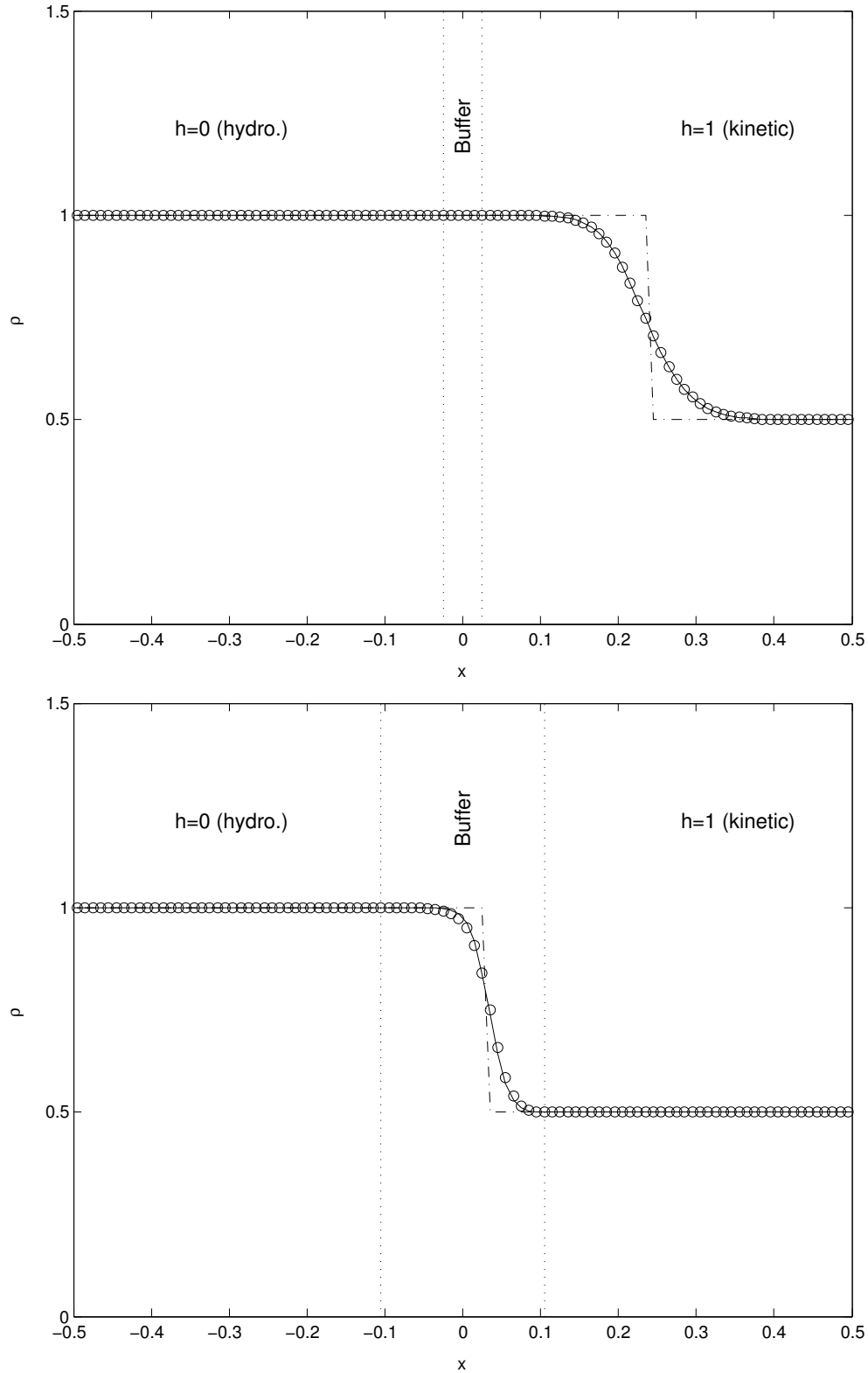
Figure 2: The numerical solution of \rho for the Jin-Xin relaxation model (27) with \varepsilon = 0.01 at t = 0.350 for the shock initial condition, with narrow (top) and large (bottom) buffer zone. The solid line is the numerical solution of model (27), while 'o' is the numerical solution of the micro-macro model (1000 grid points), and '.-' is the exact solution for the Burgers equation (full hydrodynamic limit).
