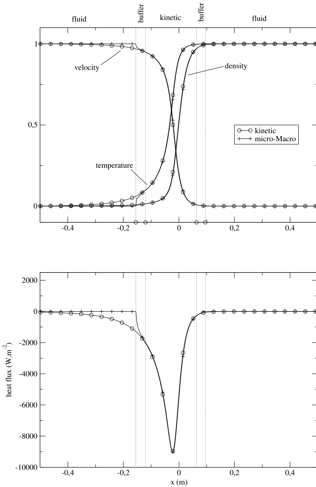
Figure 9: Density, velocity and temperature (top) and heat flux (bottom) for the stationary normal shock wave. Comparison of the full kinetic BGK equation to the micro-Macro model with a kinetic zone defined by a local Knudsen number greater than 10^{-2} .
