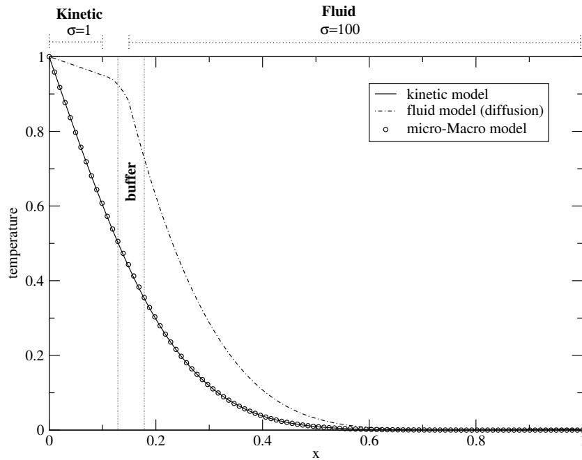
Figure 17: The numerical solution of the temperature for the radiative-heat transfer model (4.2) with at t = 0.0185 , with a buffer inside the fluid zone (top) and a buffer partially outside the fluid zone (bottom).
