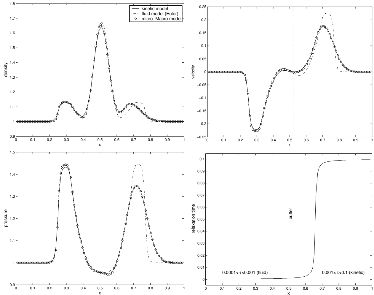
Figure 6: The numerical solution at t = 0.1103 of density (top left), velocity (top right) and pressure (bottom left) for the 1D BGK model (25) with a space dependent relaxation time (from 0.0001 to 0.1, plotted bottom right).
