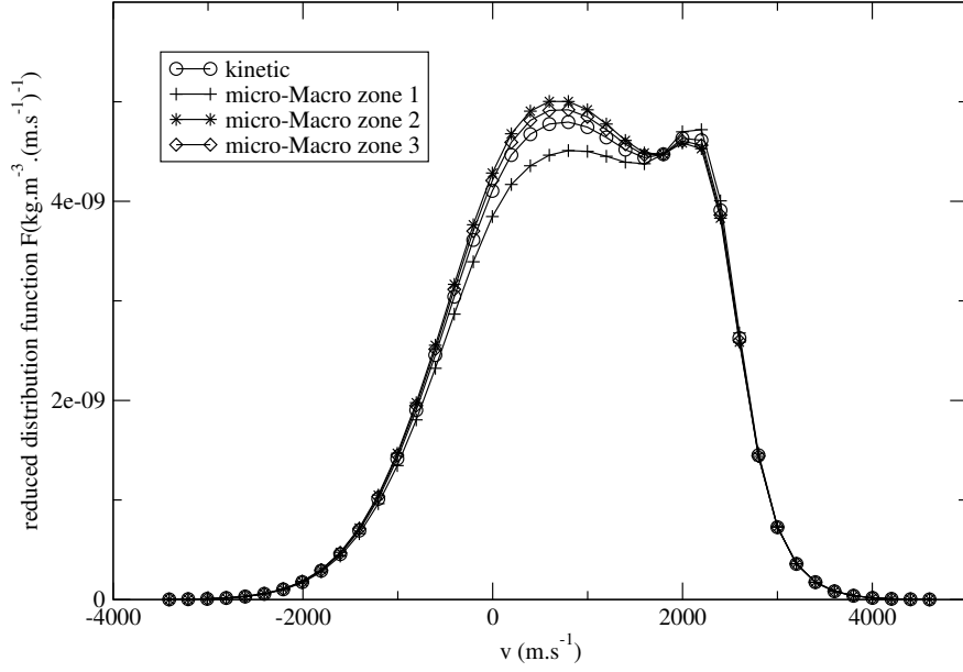
Figure 14: Stationary normal shock wave problem: reduced distribution function F(x, v) at x = 0 m (in the shock) for BGK and micro-Macro model used with three different kinetic zones (1: K
