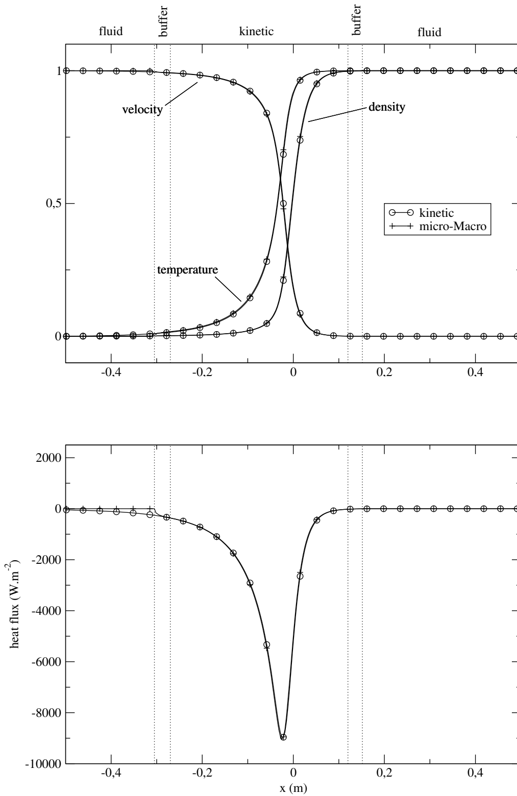
Figure 10: Density, velocity and temperature (top) and heat flux (bottom) for the stationary normal shock wave. Comparison of the full kinetic BGK equation to the micro-Macro model with a kinetic zone defined by a local Knudsen number greater than 10^{-3} .
