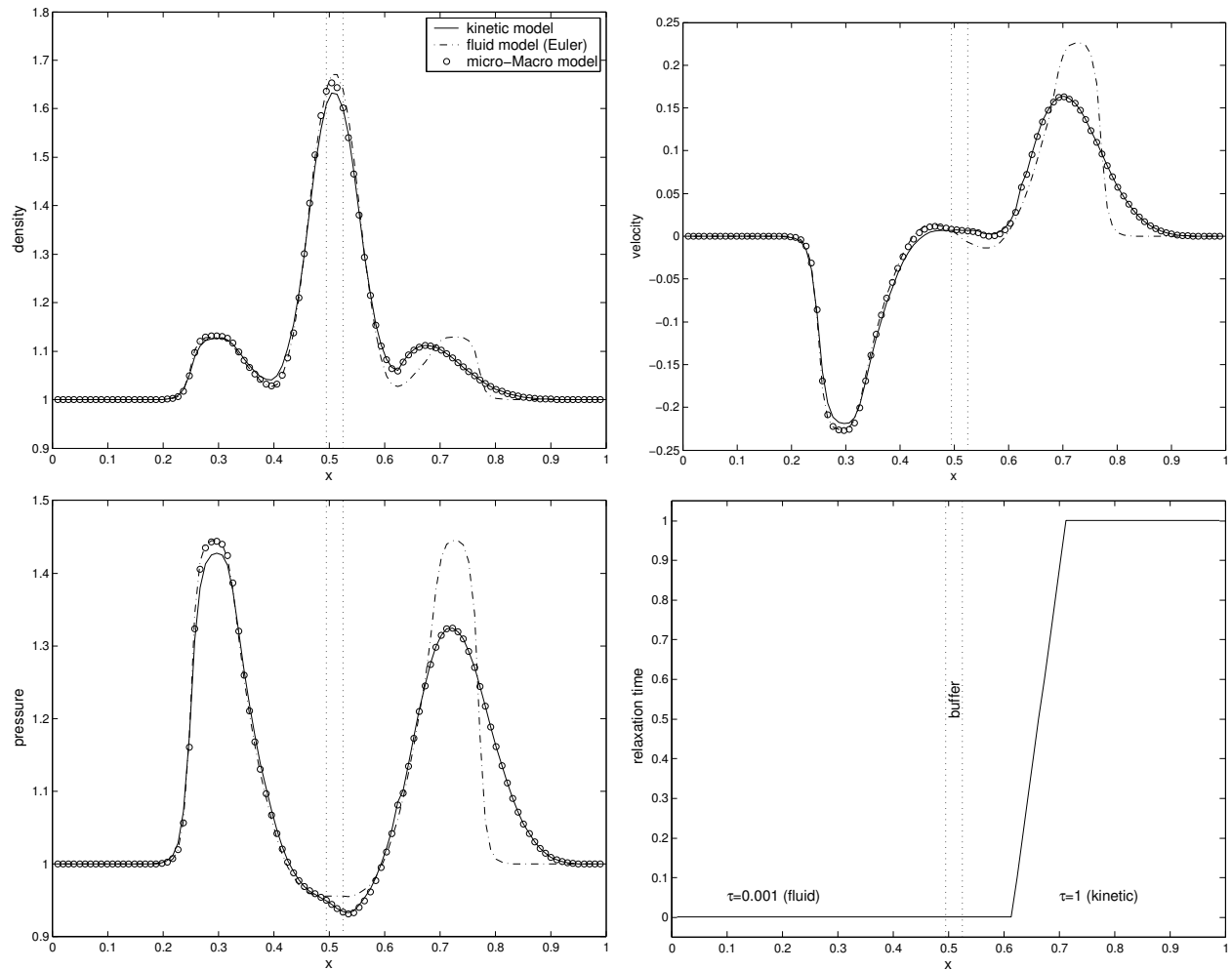
Figure 7: The numerical solution at t = 0.1103 of density (top left), velocity (top right) and pressure (bottom left) for the 1D BGK model (25) with a space dependent relaxation time (piecewise linear from 0.001 to 1, plotted bottom right).
