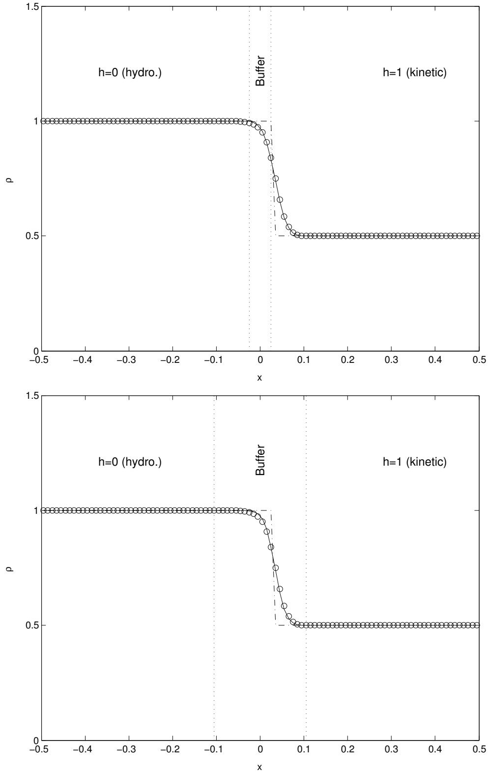
Figure 1: The numerical solution of \rho for the Jin-Xin relaxation model (27) with \varepsilon = 0.01 at t = 0.0450 for the shock initial condition, with narrow (top) and large (bottom) buffer zone. The solid line is the numerical solution of model (27), while 'o' is the numerical solution of the micro-Macro model (1000 grid points), and '-.-' is the exact solution for the Burgers equation (full hydrodynamic limit).
