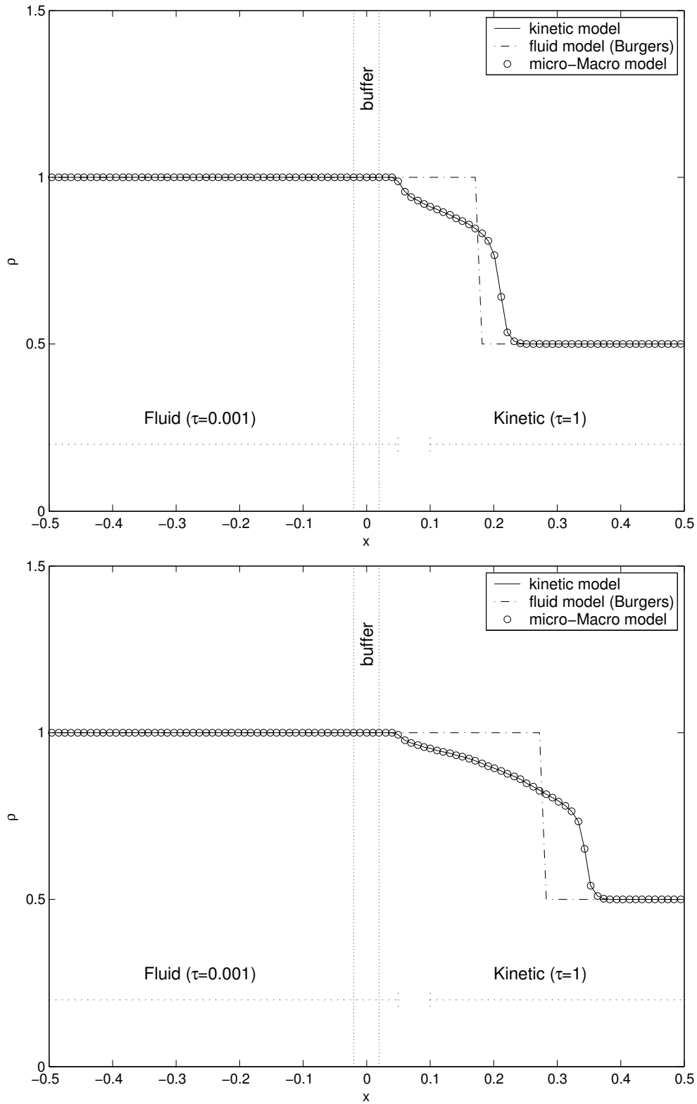
Figure 4: The numerical solution of \rho for the Jin-Xin relaxation model (27) with a space dependent relaxation time (from 0.001 to 1) at t = 0.4773 (top) and t = 0.5909 (bottom).
