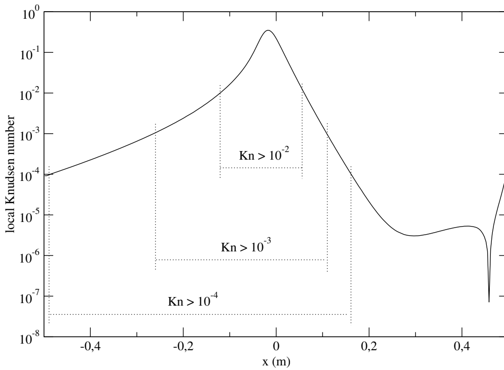
Figure 8: Local Knudsen number for the stationary normal shock wave (in log scale). The three zones where the kinetic upscaling will be used are represented by dotted lines.
