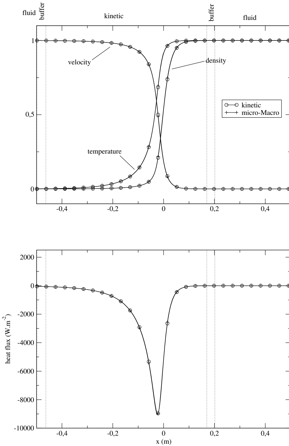
Figure 11: Density, velocity and temperature (top) and heat flux (bottom) for the stationary normal shock wave. Comparison of the full kinetic BGK equation to the micro-Macro model with a kinetic zone defined by a local Knudsen number greater than 10^{-4} .
