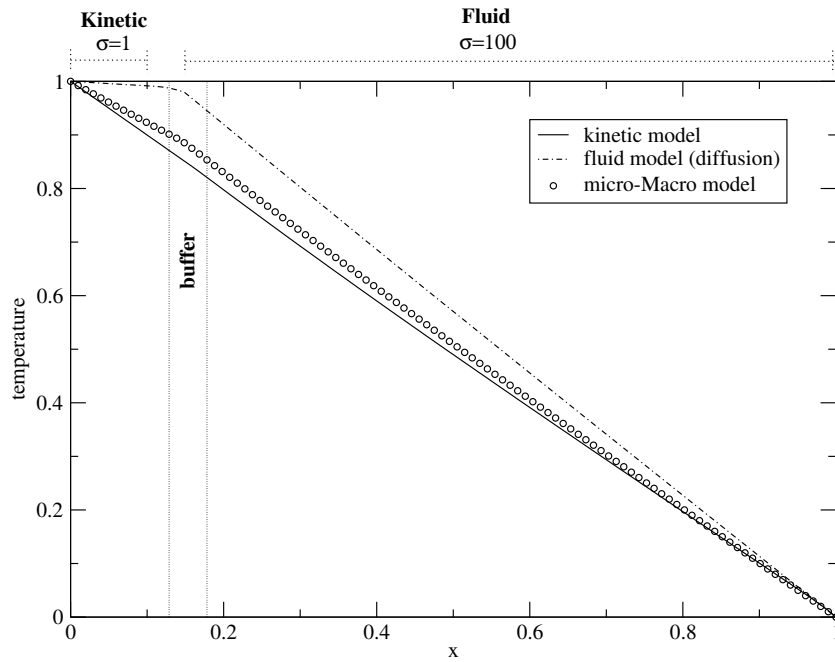
Figure 18: The numerical solution of the temperature for the radiative-heat transfer model (4.2) at steady state, with a buffer inside the fluid zone (top) and a buffer partially outside the fluid zone (bottom).
