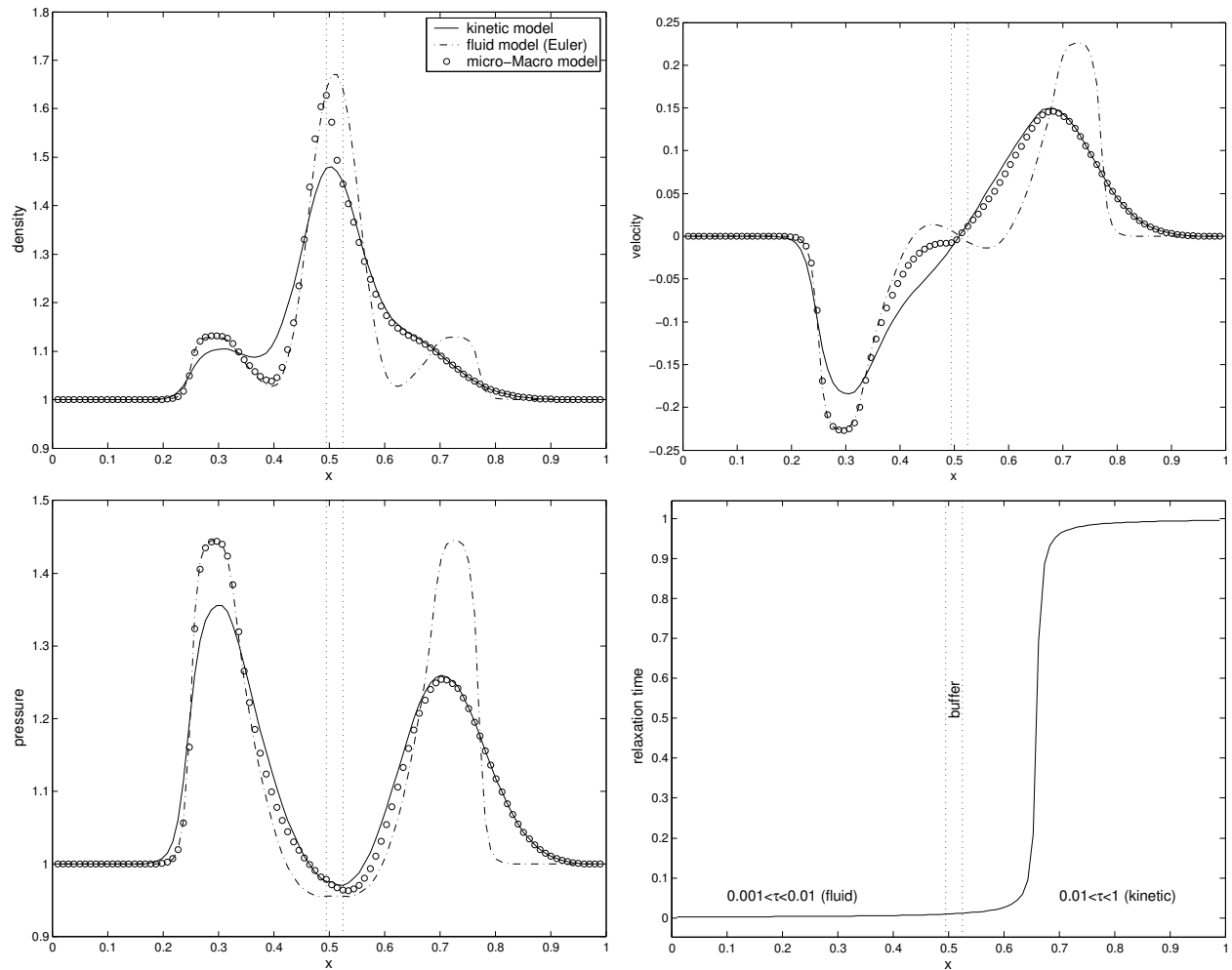
Figure 5: The numerical solution at t = 0.1103 of density (top left), velocity (top right) and pressure (bottom left) for the 1D BGK model (25) with a space dependent relaxation time (from 0.001 to 1, plotted bottom right).
