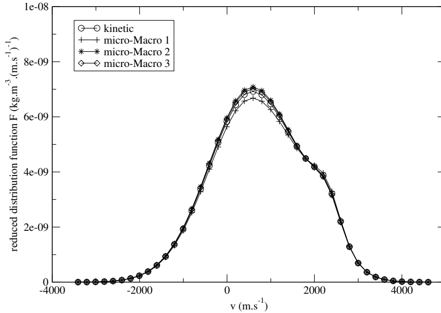
Figure 15: Stationary normal shock wave problem: reduced distribution function F(x, v) at x = 0.0117 m (right part of the shock) for BGK and micro-Macro model used with three different kinetic zones (1: Kn > 10^{-2} , 2: Kn > 10^{-2} , 3: Kn > 10^{-2} ).
