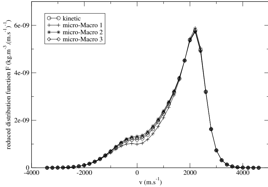
Figure 13: Stationary normal shock wave problem: reduced distribution function F(x, v) at x = -0.0217 m (left part of the shock) for BGK and micro-Macro model used with three different kinetic zones (1: Kn > 10^{-2} , 2: Kn > 10^{-2} , 3: Kn > 10^{-2} ).
