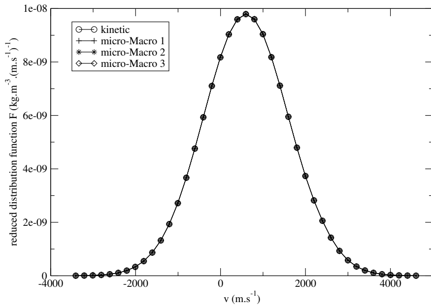
Figure 16: Stationary normal shock wave problem: reduced distribution function F(x, v) at x = 0.0717 m (downstream) for BGK and micro-Macro model used with three different kinetic zones (1: Kn > 10^{-2} , 2: Kn > 10^{-2} , 3: Kn > 10^{-2} ).
