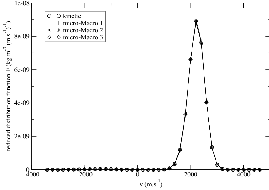
Figure 12: Stationary normal shock wave problem: reduced distribution function F(x, v) at x = -0.1383 m (upstream) for BGK and micro-Macro model used with three different kinetic zone
