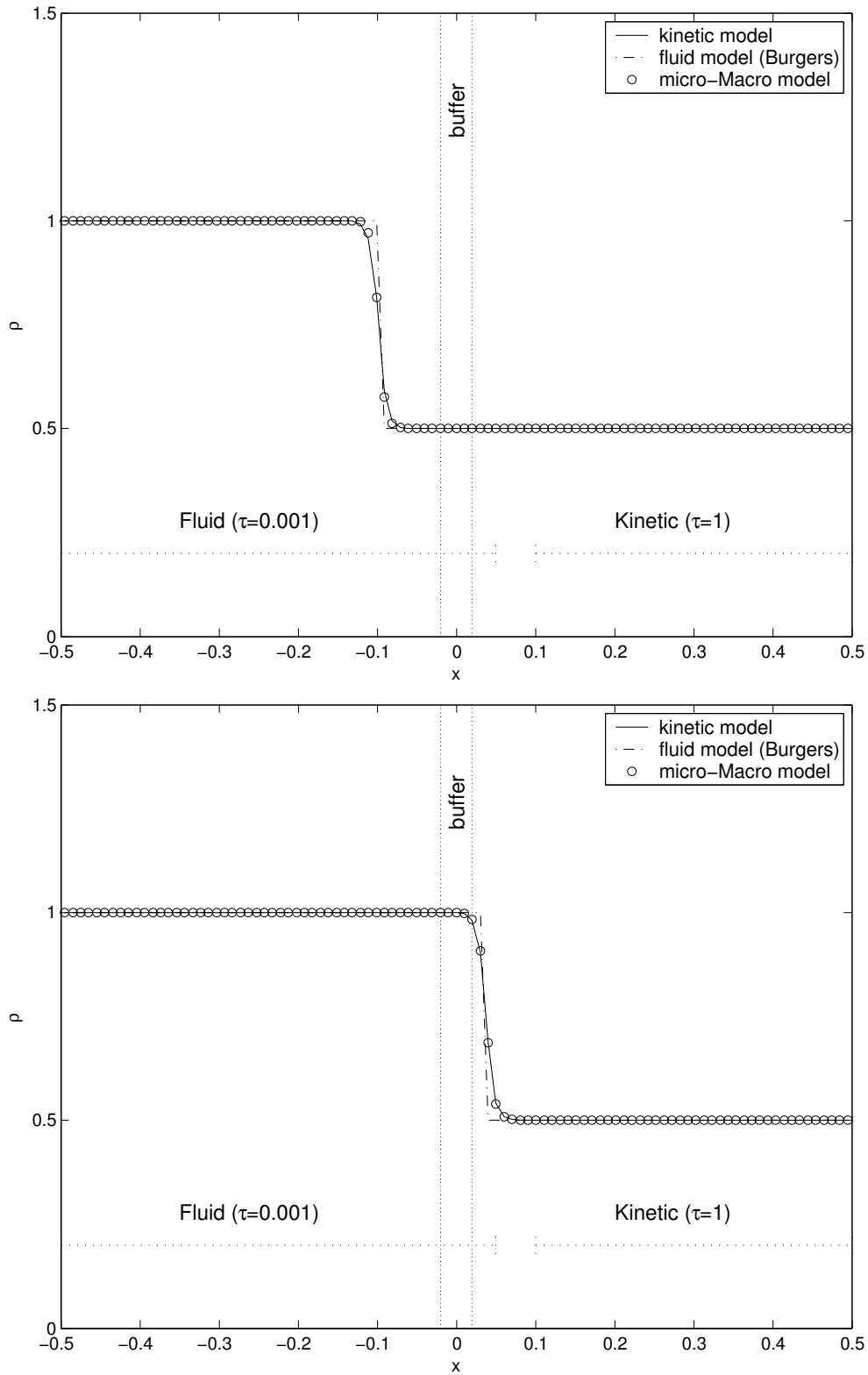
Figure 3: The numerical solution of \rho for the Jin-Xin relaxation model (27) with a space dependent relaxation time (from 0.001 to 1) at t = 0.0909 (top) and t = 0.2773 (bottom).
