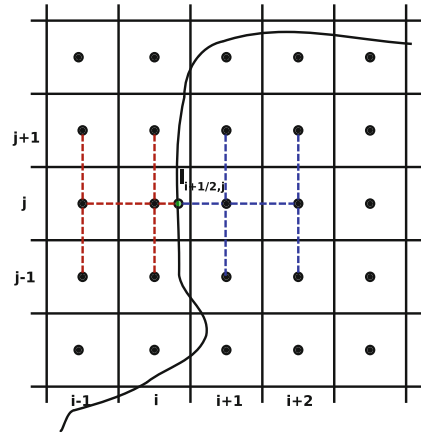
(b) Discretization of \nabla U at the interface: non-stabilized stencil.
