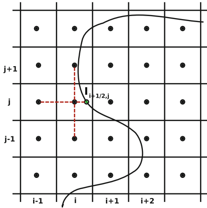
(a) Discretization of the Laplacian on the points at the interface.
