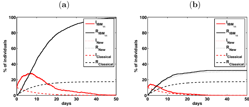
Figure 8: Comparison of simulations of the \text{IBM}_{11} (solid curves), the new SIR model (3.2) (dotted curves), and the classical SIR model (1.1) (dashed curves) with \beta = \beta_S and a non-fully random graph of connection at time t = 0 . Here S = 0.9 , I = 0.1 , S_c = S at time t = 0 . T_R = 5 and \beta_S = 0.1 are fixed. (a) T_C = 10 and p_S = \beta_S T_C = 1 . (b) T_C = 0.1 and p_S = \beta_S T_C = 0.1 .
