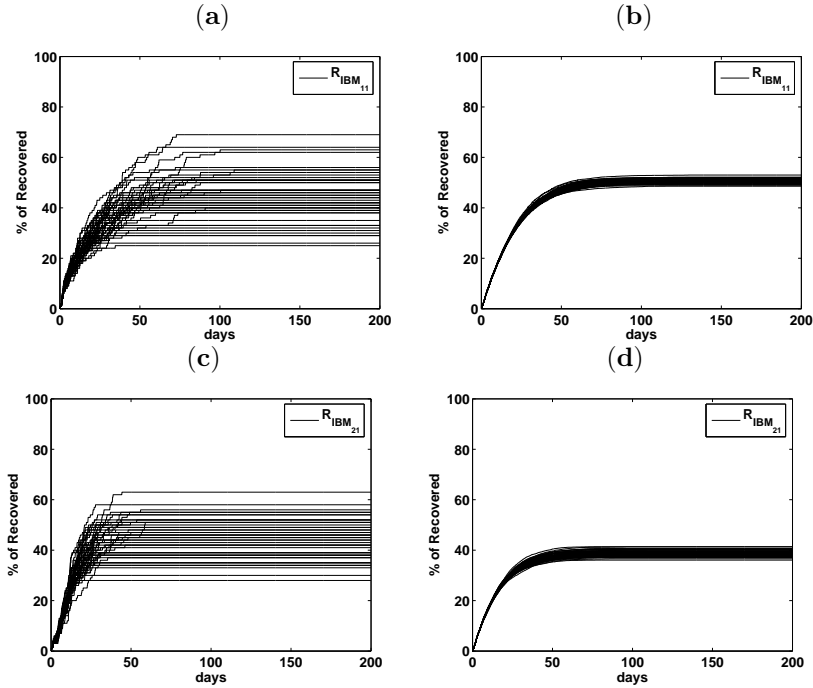
Figure 7: Simulations of the recovered class in the IMB. In (a) and (b) the IBM_{11} was run 50 times to simulate the transmission at the end of the contact for N = 100 and N = 10000 , respectively. In (c) and (d) the IBM_{21} was run 50 times to simulate the transmission at the beginning of the contact for N = 100 and N = 10000 , respectively. All parameters are the same as in Fig. 6.
