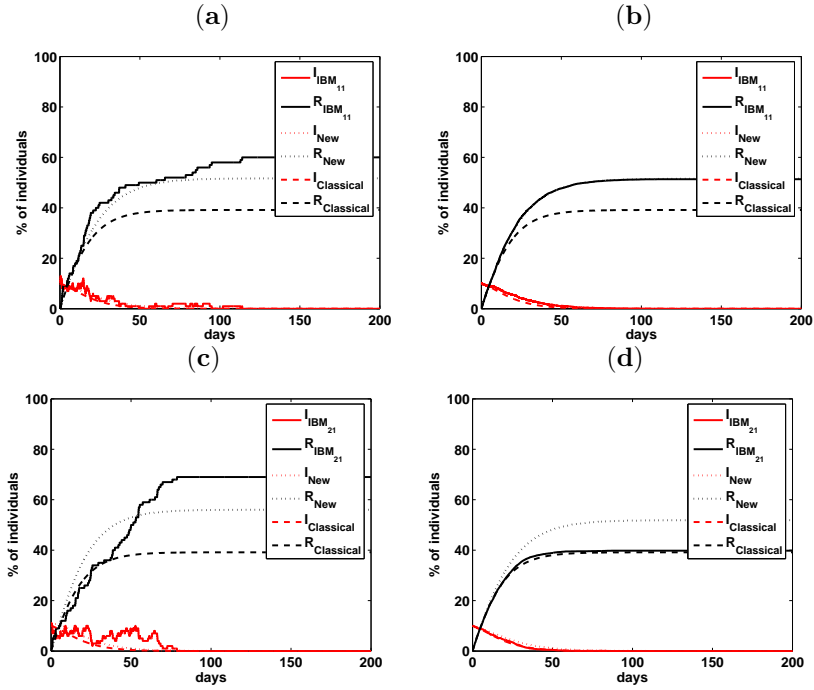
Figure 6: Comparison of simulations of the IBM (solid curves), the new SIR model (3.2) (dotted curves), and the classical SIR model (1.1) (dashed curves) with \beta = \beta_S, I = (1/10)N, S = (9/10)N with S_c = SI/(S + I + R) at time t = 0 . T_C = 5, T_R = 5, \beta_S = 0.2 and p_S = \beta_S T_C = 1 were fixed. \nu_c = 1/T_C = 1/5, \nu_R = 1/T_R = 1/5 . In (a) and (b) the IBM_{11} was run to simulate the transmission at the end of the contact for N = 100 and N = 10000 , respectively. In (c) and (d) the IBM_{21} was run to simulate the transmission at the beginning of the contact for N = 100 and N = 10000 , respectively.
