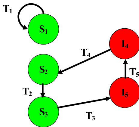
Figure 1: Diagram of the contact network at a given time t \geq 0 . The first S -individual ( S_1 ) only contacts with himself. The second S -individual ( S_2 ) chooses to contact with a third S -individual ( S_3 ) who in turn contacts with an I -individual ( I_5 ). I_5 contacts another I -individual ( I_4 ) who in turn chooses S_2 for contact.
