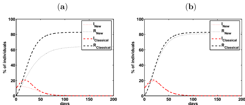
Figure 11: Comparison of the new SIR model (4.10) (dotted curves) and the classical SIR model (1.1) (dashed curves) with \beta = \beta_S . (a) The total number of recovered individuals in the new and classical SIR models are significantly different as time increases. (b) The solution of the new SIR model converges to the solution of the classical SIR model. Here S/N = 0.9 , I/N = 0.1 , S_c = I_c = SI/N at time t = 0 , T_R = 10 and \beta_I = 0.2 (a) T_C = 5 and p_I = \beta_I T_C = 1 . (b) T_C = 0.5 and p_I = \beta_I T_C = 0.1
