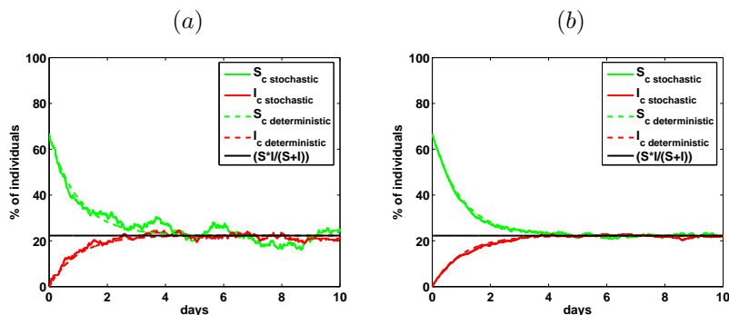
Figure 2: The comparison between solutions of the ordinary differential equation model (2.1) and Monte Carlo simulations of the model. The solutions of the stochastic model converge to the equilibrium solutions of the ODE model. Here \nu_c = 1 , I = N/3 , S = 2N/3 , I_c = 0 and S_c = S at time t = 0 . (a) N = 200 and (b) N = 2000 .
