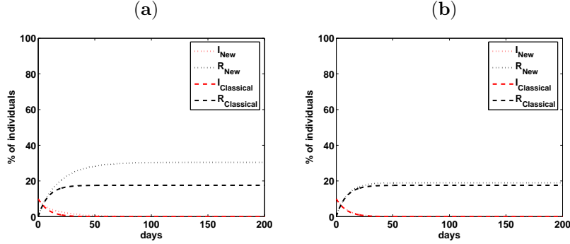
Figure 5: Comparison of the new SIR model (3.2) (dotted curves) and classical SIR model (1.1) (dashed curves) with \beta = \beta_S = p_S/T_C , S = 0.9 , I = 0.1 , S_c = SI/(S + I + R) at time t = 0 . T_R = 5 and \beta_S = 0.1 were fixed. (a) T_C = 10 and p_S = \beta_S T_C = 1 . (b) T_C = 1 and p_S = \beta_S T_C = 0.1 . In both cases the solutions of the new SIR model converge to the solutions of the classical SIR model.
