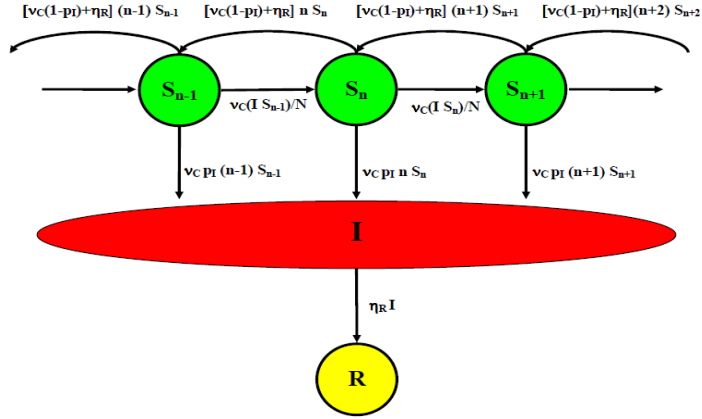
Figure 10: Flux diagram of model (4.4).
