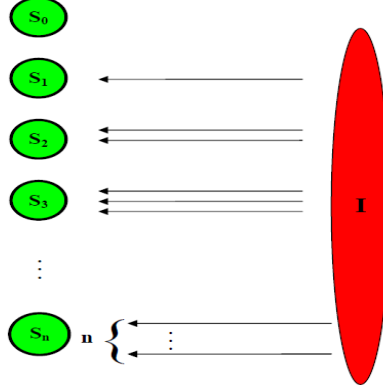
Figure 9: Structured diagram of the population in term of contacts indicating the number of S -individuals chosen for a contact by I -individuals. S_n is the group of S -individuals which has been chosen n times by I -individuals, where n = 0, 1, 2, \dots
