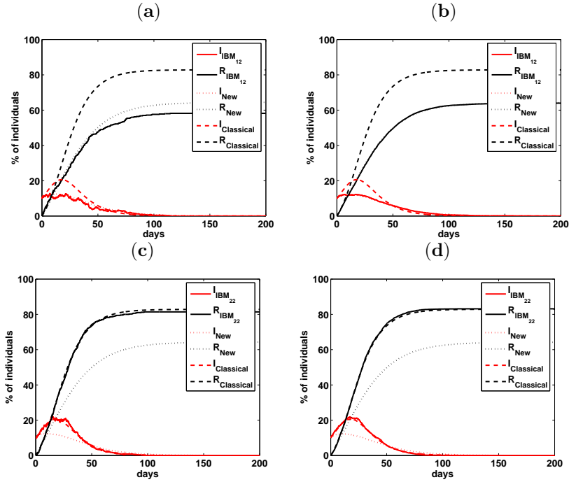
Figure 12: Comparison of the IBM (solid curves), the new SIR model (4.10) (dotted curves), and the classical SIR model (1.1) (dashed curves) with \beta = \beta_I , S/N = 0.9 , I/N = 0.1 , S_c = I_c = SI/N at time t = 0 . T_R = 10 , \beta_I = 0.2 , T_C = 5 , and p_I = \beta_I T_C = 1 are fixed. In (a) and (b) the IBM 12 was run to simulate the transmission at the end of the contact for N = 100 and N = 10000 , respectively. In (c) and (d) the IBM 22 was run to simulate the transmission at the beginning of the contact for N = 100 and N = 10000 , respectively.
