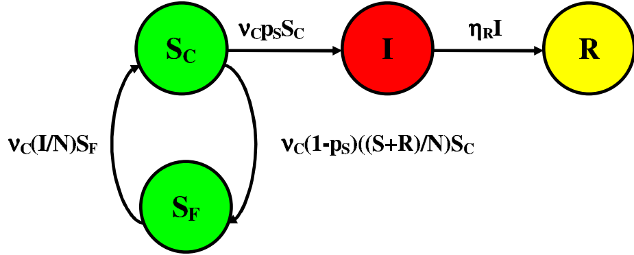
Figure 4: The flux diagram of model (3.2).
