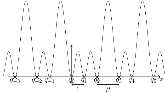
FIGURE 3. Graph of the potential V for \alpha = 1/\sqrt{5} and \rho = \sqrt{3}
