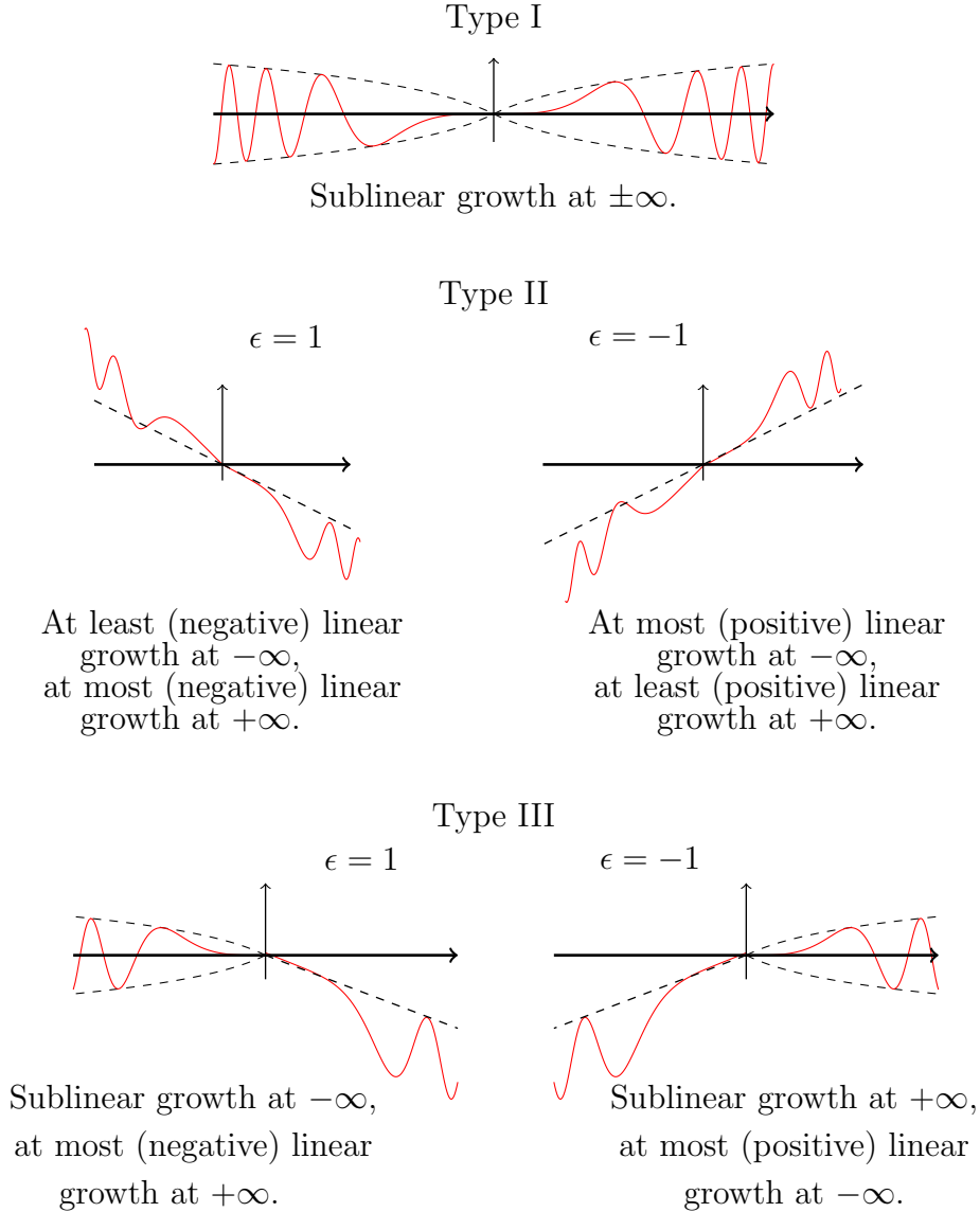
FIGURE 1. The different possible asymptotic behaviors of weak KAM solutions
