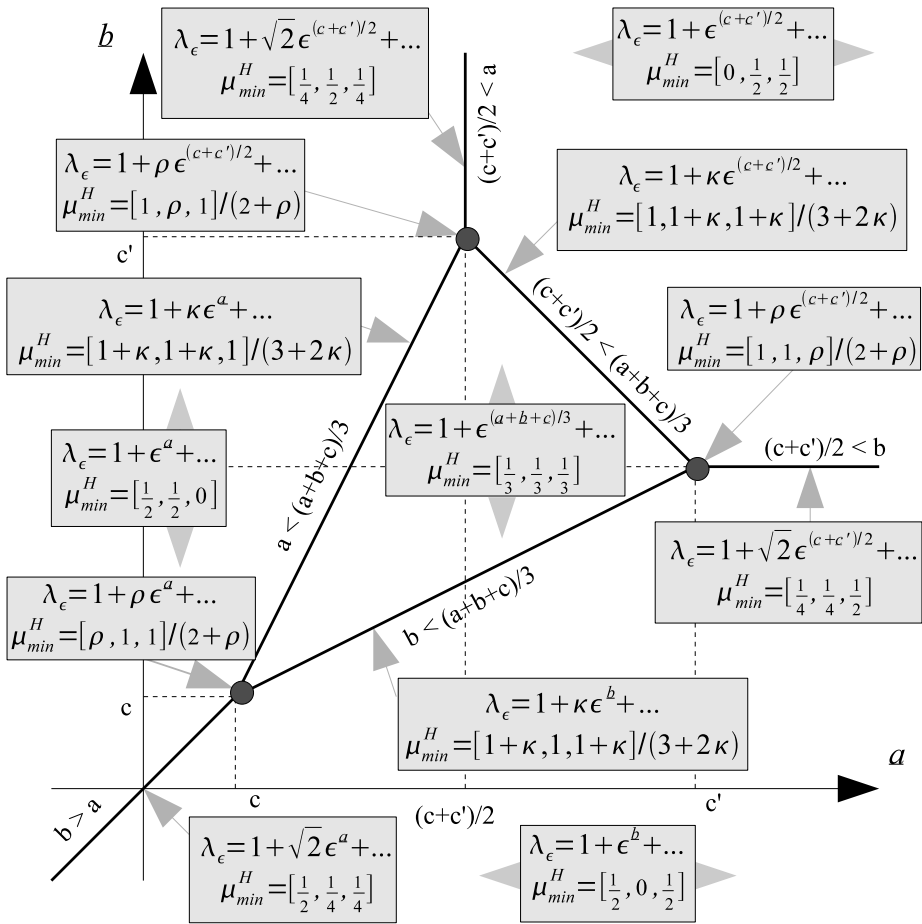
Fig. 8 Phase diagram for a 3 \times 3 matrix with three irreducible components. We assume c < c' . The zero-temperature Gibbs measure is a barycenter of the three periodic measures \delta_{(1\infty)} , \delta_{(2\infty)} and \delta_{(3\infty)} . The constants \rho and \kappa are solutions of \rho^2 - \rho - 1 = 0 and \kappa^3 - \kappa - 1 = 0 . The exact values of these constants are \rho = \frac{1}{2}(1 + \sqrt{5}) and \kappa = \sqrt[3]{\frac{1}{2}(1 - \sqrt{23/27})} + \sqrt[3]{\frac{1}{2}(1 + \sqrt{23/27})}
