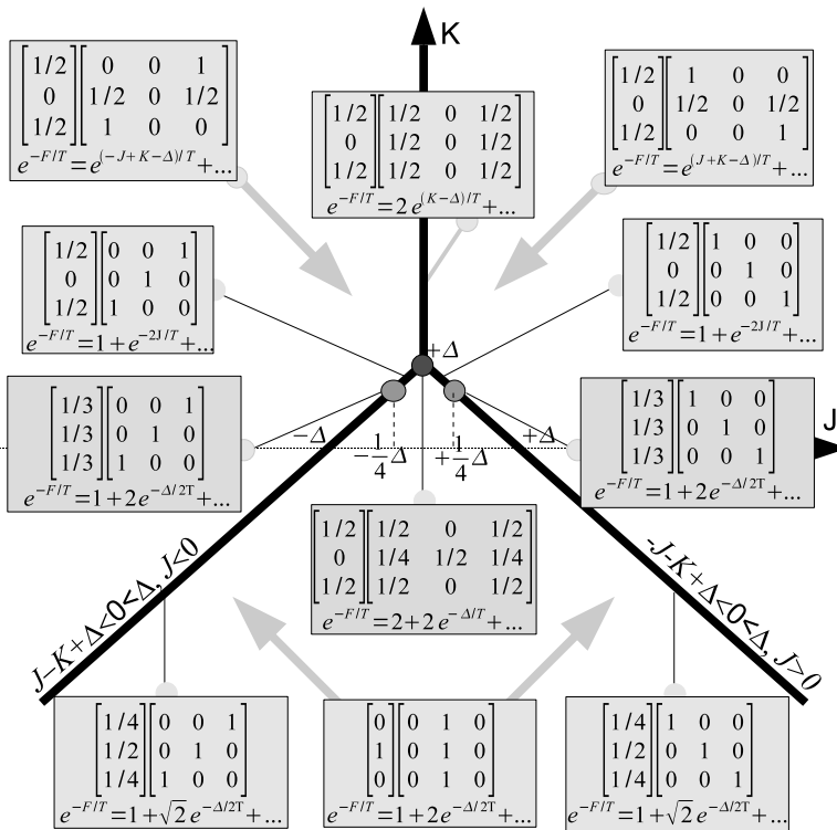
Fig. 3 Phase diagram of the BEG model at zero temperature for \Delta > 0 . The Markov chain structure (\pi_\infty, Q_\infty) at zero temperature and the Puiseux series expansion of the free energy F = \bar{H}_\beta is shown for each phase
