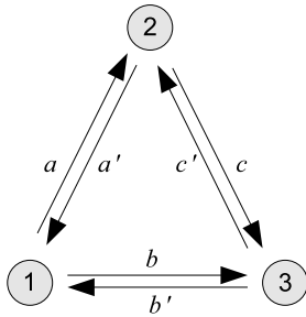
Fig. 7 Graph of interactions and minimizing cycles of M_\epsilon - \text{Id}
