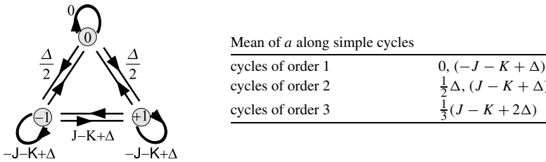
Fig. 2 Graph of interactions and determination of minimizing cycles (a cycle of minimizing mean) in the BEG model
