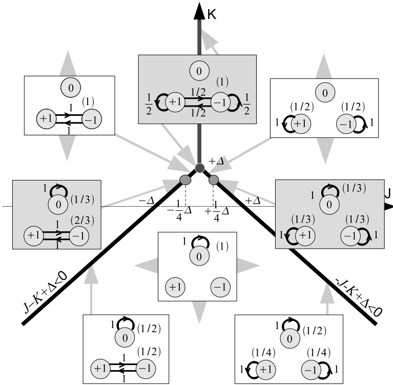
Fig. 4 Phase diagram of the BEG model at zero temperature for \Delta > 0 . Numbers in parentheses indicate the weight of each indecomposable (ergodic) Markov chain which contributes to the zero-temperature Gibbs measure
