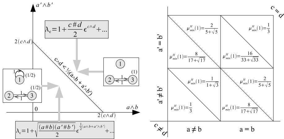
Fig. 5 Phase diagram for a 3 \times 3 matrix with two irreducible components: part I. In the left diagram , numbers in parentheses indicate the weight of each irreducible components. In the right diagram , the value of \mu_{\min}^H(1) is shown for the case c \wedge d = \frac{1}{2}(a \wedge b + a' \wedge b')
