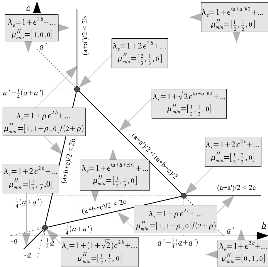
Fig. 6 Phase diagram for a 3 \times 3 matrix with two irreducible components: part II. We assume a < a' . The zero-temperature Gibbs measure is a barycenter of the periodic measures \delta_1 and \delta_2
